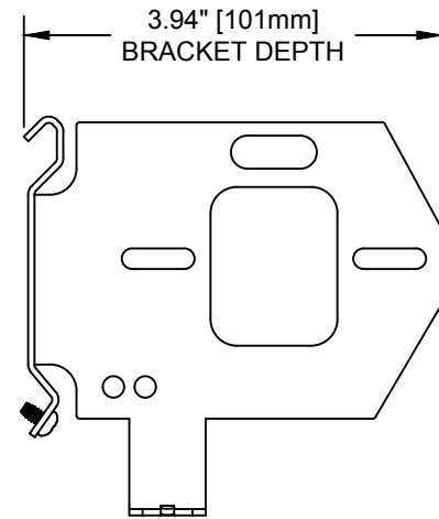
ELEVATION VIEW
