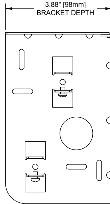
ELEVATION VIEW
