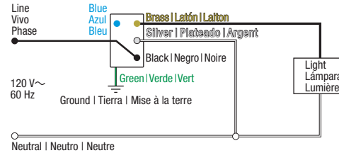
Image #17 — Dimmer with One Black Screw, One Brass Screw, One Blue Screw, and One Silver Screw in a Single Pole Application
