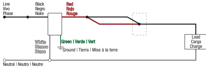
Image #48 — Dimmer with One Black Wire, One Red Wire and one White Wire in a 3-Way Application with a Pico Remote (continued)
