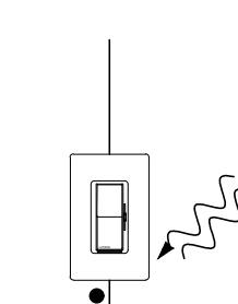
DVRF-6L-XX 120V~ 50/60 Hz DIVA SMART DIMMER FOR CASÉTA LED, CFL, INC & HAL LOADS ON/OFF BUTTON CONTROL W/ SLIDER FOR DIMMING & STATUS LED SHOWN WITH CW-1-WH CLARO WALLPLATE (1 GANG US BACKBOX BY OTHERS) LOCATION TBD
