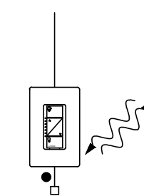
PD-6WCL-WH 120V~ 50/60 Hz CASÉTA ORIGINAL IN-WALL DIMMER LED, CFL, INC, & HAL LOADS 2 BUTTON CONTROL WITH RAISE/LOWER SHOWN WITH CW-1-WH CLARO WALLPLATE (1 GANG US BACKBOX BY OTHERS) LOCATION TBD
